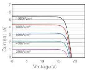
Current Voltage Curve
