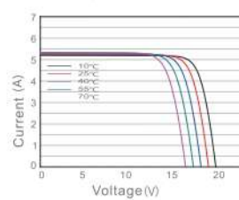
Current Voltage Curve
